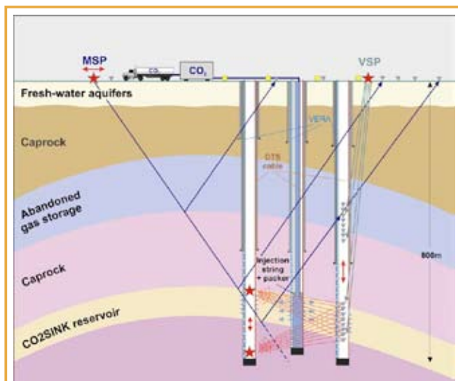
Figure 2. Schematic concept of Ketzin geology, drilling, and geophysical monitoring including moving source seismic profiling (MSP), vertical seismic profiling (VSP), cross-hole seismics, surface 3D seismics, and surface and cross-hole geoelectrics using a permanently installed Vertical Electrical Resistivity Array (VERA), and Distributed Temperature Sensing (DTS) (from Förster et al., 2006).
