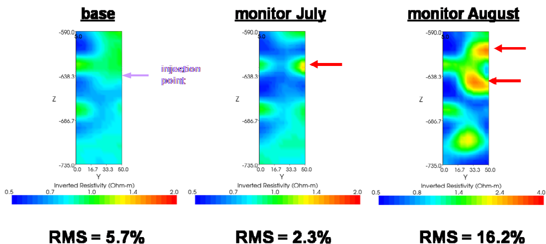
Fig. 5. Evaluation of 2D-slices as preliminary results of resistivity mapping of the reservoir in the near-borehole area. The inversion was carried out using the EarthImager3D software.
