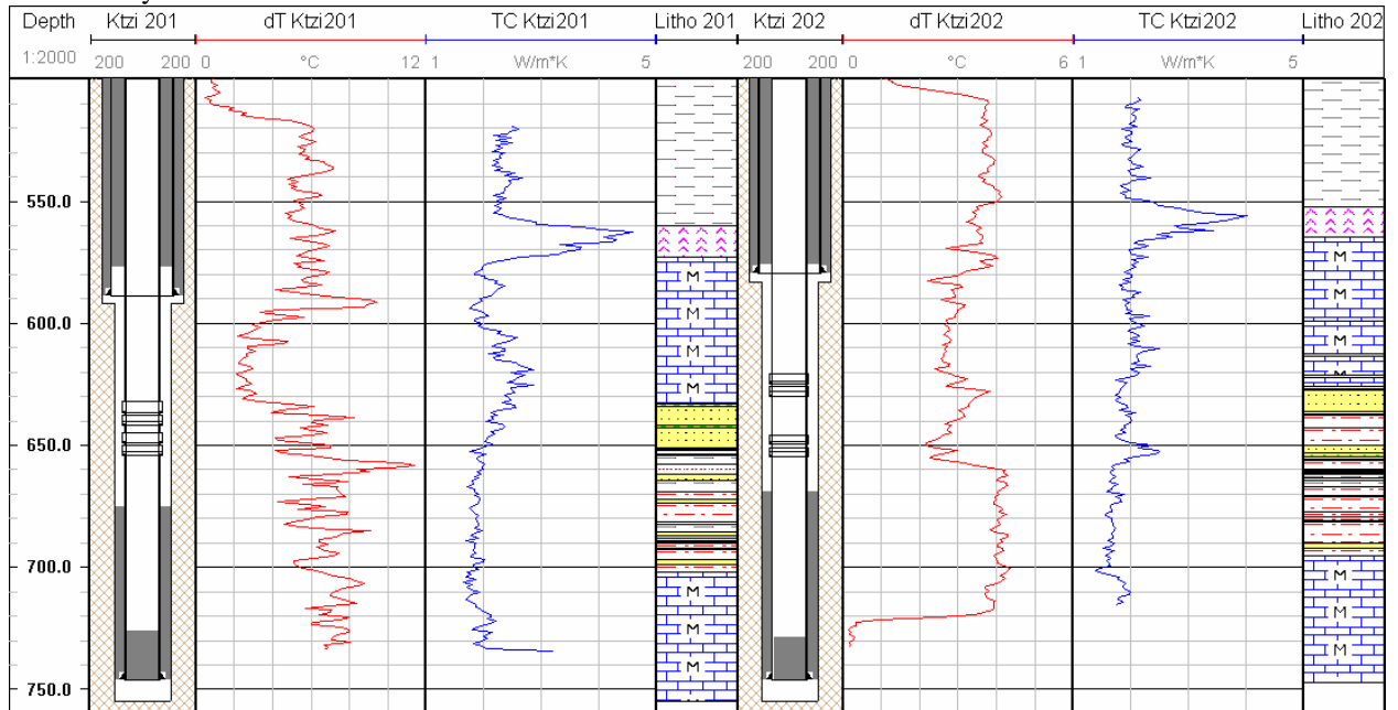
Figure 4. Well logs for Ktzi201 and Ktzi202 showing temperature changes (dT) during DTPS heating and calculated thermal conductivities (TC) along with well layouts and lithologies [after Förster et al., 2008]. Note that at a depth of ~560 m there is an anhydrite rich marker bed which is indicated by elevated thermal conductivities.
